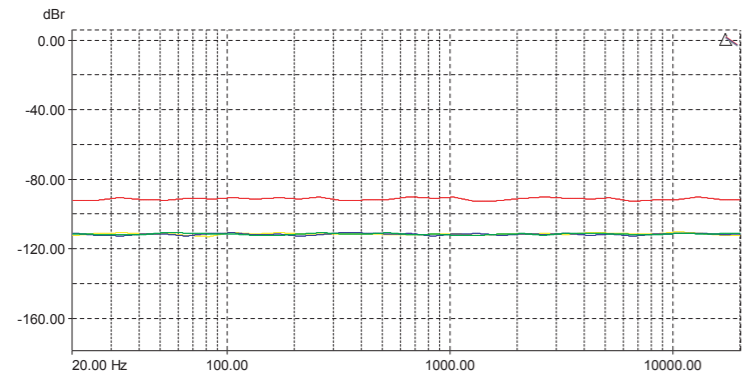
Figure 6.5 Common mode rejection @ 20 Hz --> 20 kHz (measurement of a typical performance)
